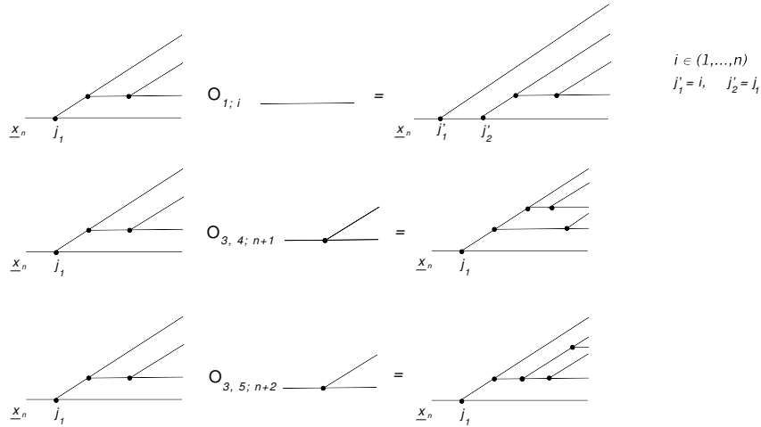
Figure 5.2. Examples of composition of trees: in \overline{\mathcal{D}} \circ_{\underline{k};i} \overline{\mathcal{G}} the indices k_0, i indicate to which line of \overline{\mathcal{D}} (and between which nodes) has to be attached the root of \overline{\mathcal{G}} , and the k_1, \dots, k_q indicate how to order the q nodes of the subtree \overline{\mathcal{G}} in the resulting tree.
