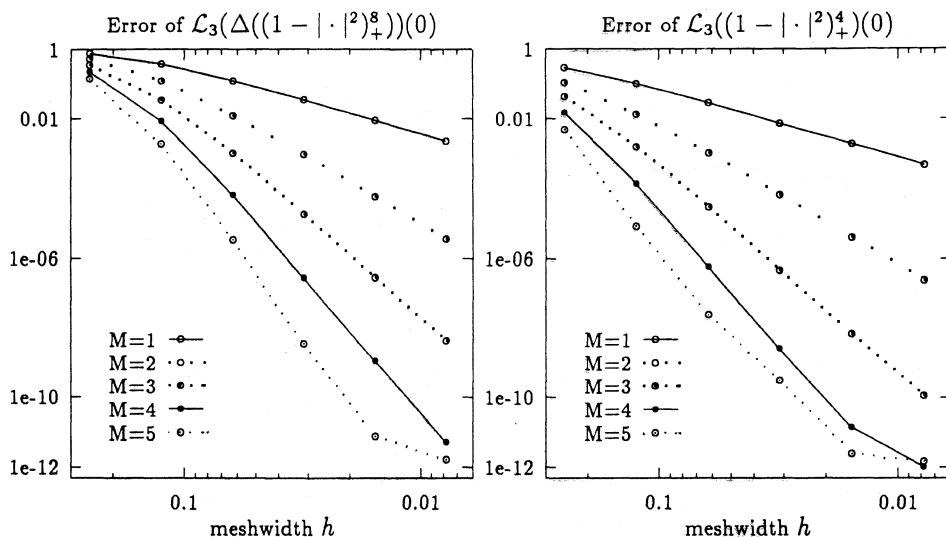
Fig. 1. – Cubature error for the Newton potential using different generating functions \eta_{2M} and the fixed parameter \varpi = 3 .
