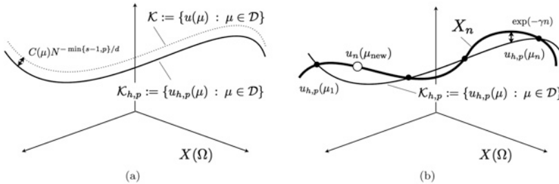
Fig. 1 – (a) Low-dimensional manifold \mathcal{K}_{h,p} on which the field variable resides and (b) approximation of a new solution at \mu_{\text{new}} with the “snapshots” u_{h,p}(\mu_m) , 1 \leq m \leq n .
